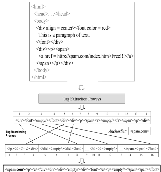
Procedure flow of Structure Abstraction Generation
